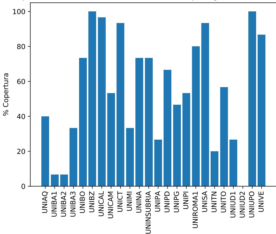
Copertura PD (Parallel and Distributed Computing): T1=5.0 T2=10.0
