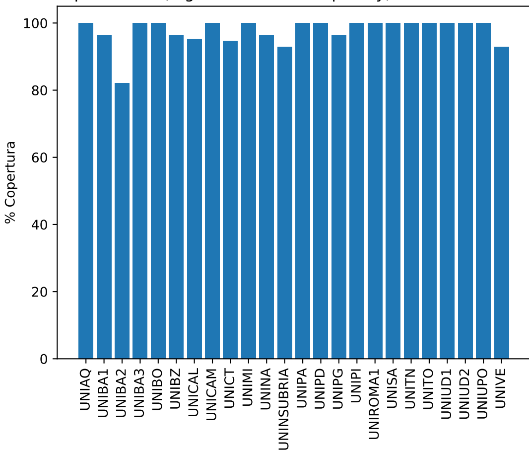
Copertura AL (Algorithms and Complexity): T1=19.0 T2=9.0
