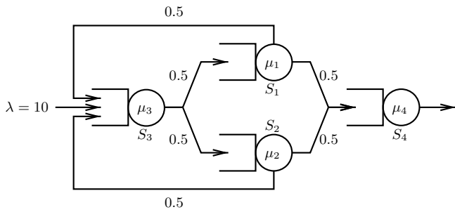
Figure 7: Open QN. Service rates are \mu_1 = \mu_2 = 25 , \mu_3 = 50 , \mu_4 = 30
